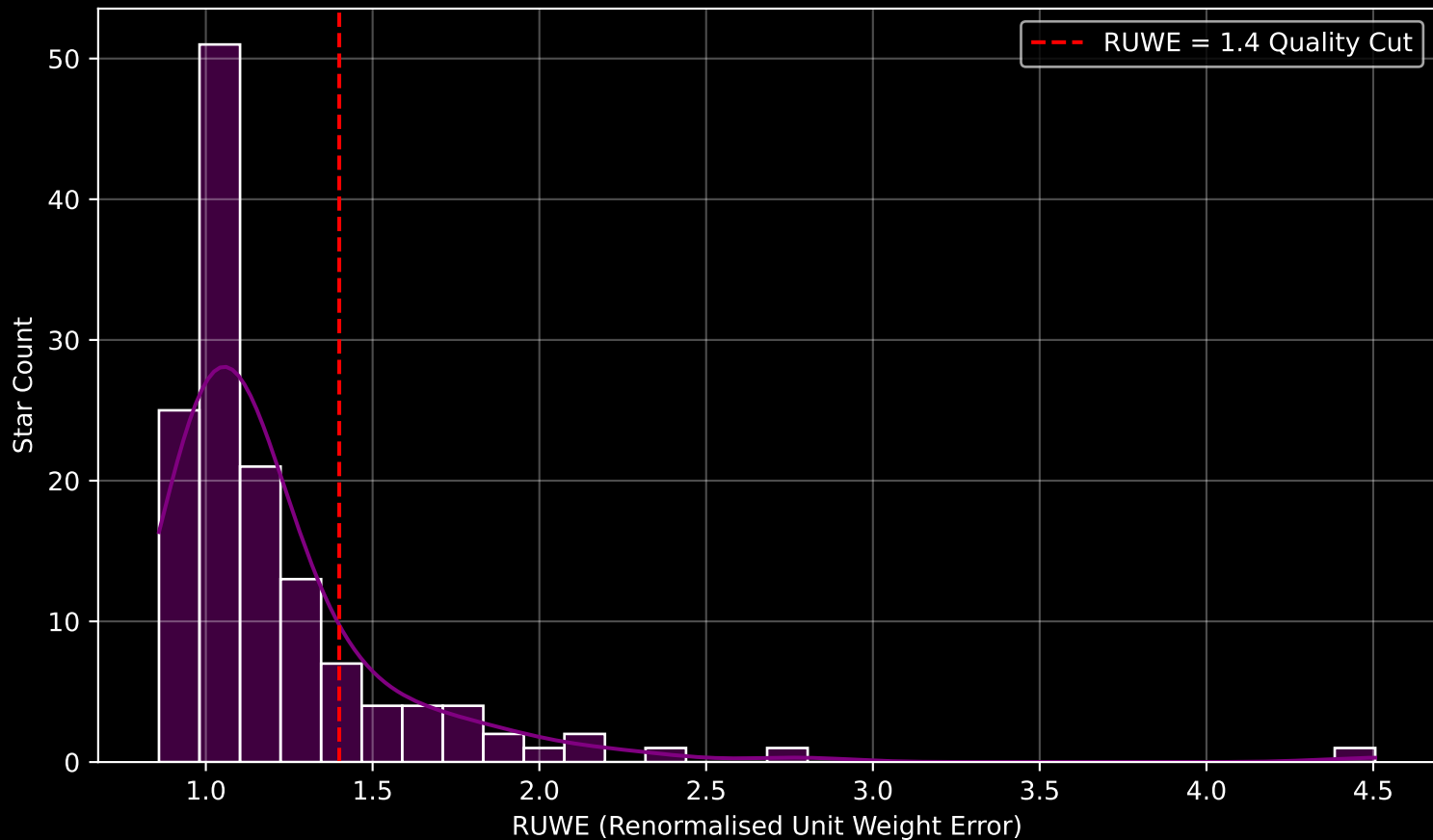
GAPOGEE DR17 Field [040+38_MGA] RUWE Distribution (n= 137)
