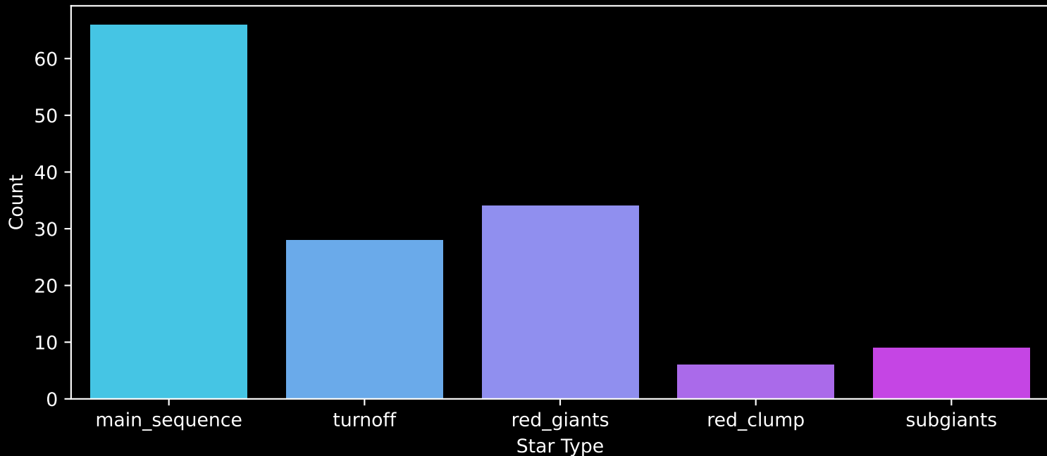
APOGEE DR17 Field: [040+38_MGA] Count plot of Star Type
