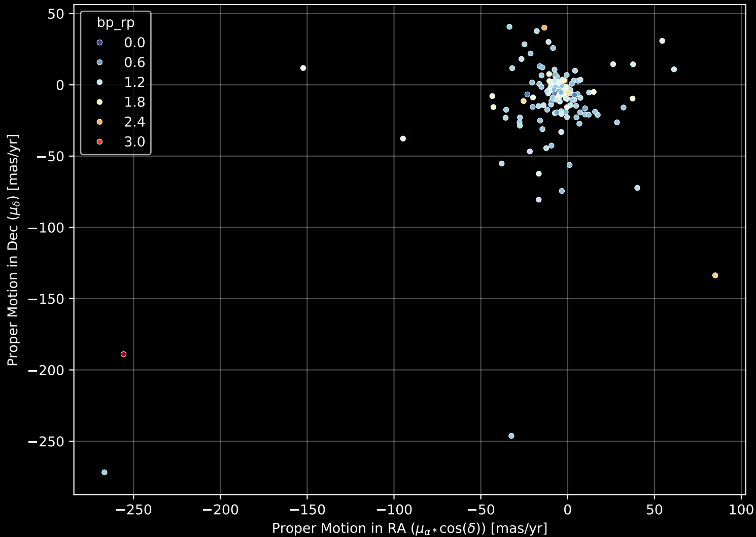
APOGEE DR17 Field: [040+38_MGA] Proper Motion Diagram (n= 143)
