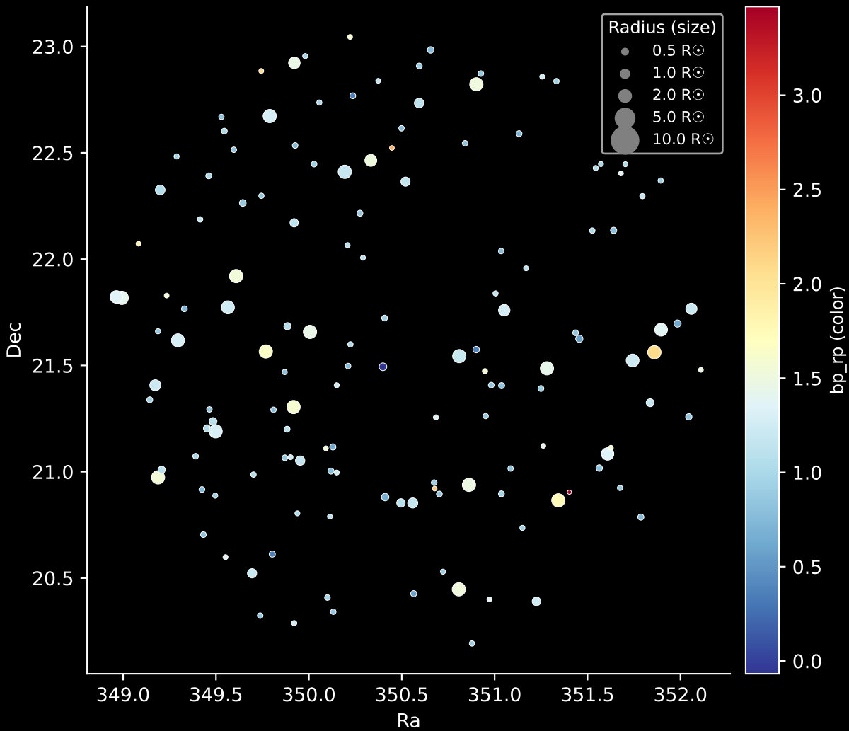
APOGEE DR17 Field: [040+38_MGA] Stars: 143
