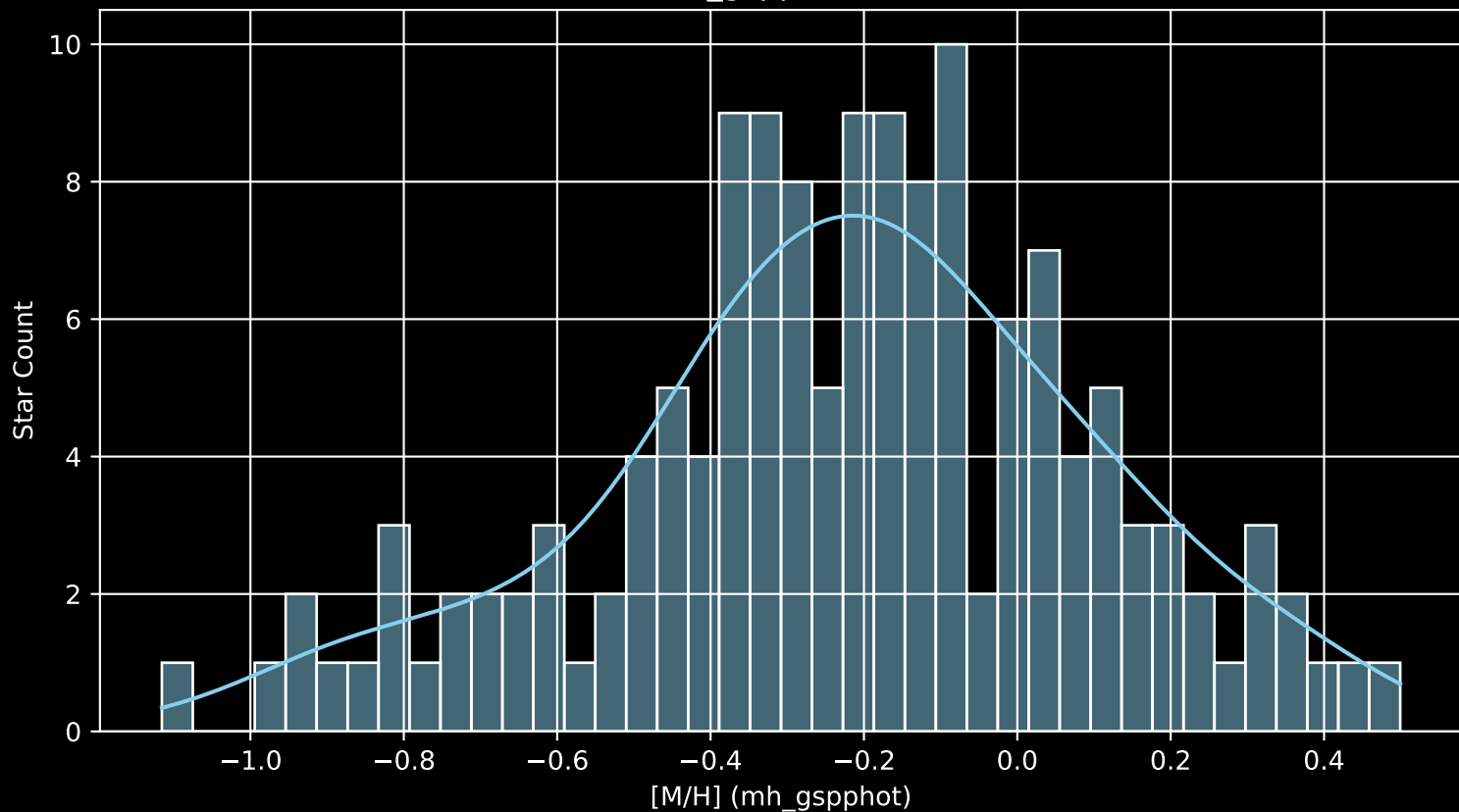
APOGEE DR17 Field: [040+38_MGA [M/H] (mh_gspphot) (n= 143)
