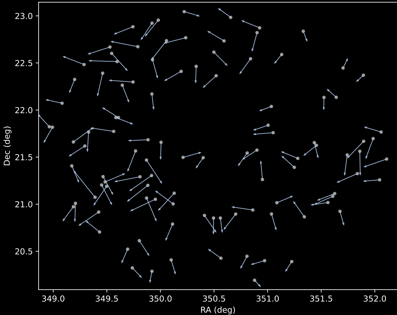
APOGEE DR17 Cluster 1 Proper Motion Vectors (n=105)
