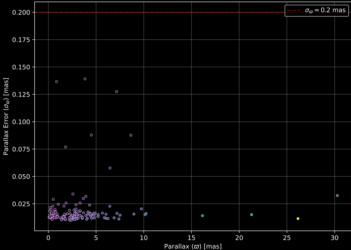
APOGEE DR17 Field: [040+38_MGA] Parallax Quality (n= 143)
