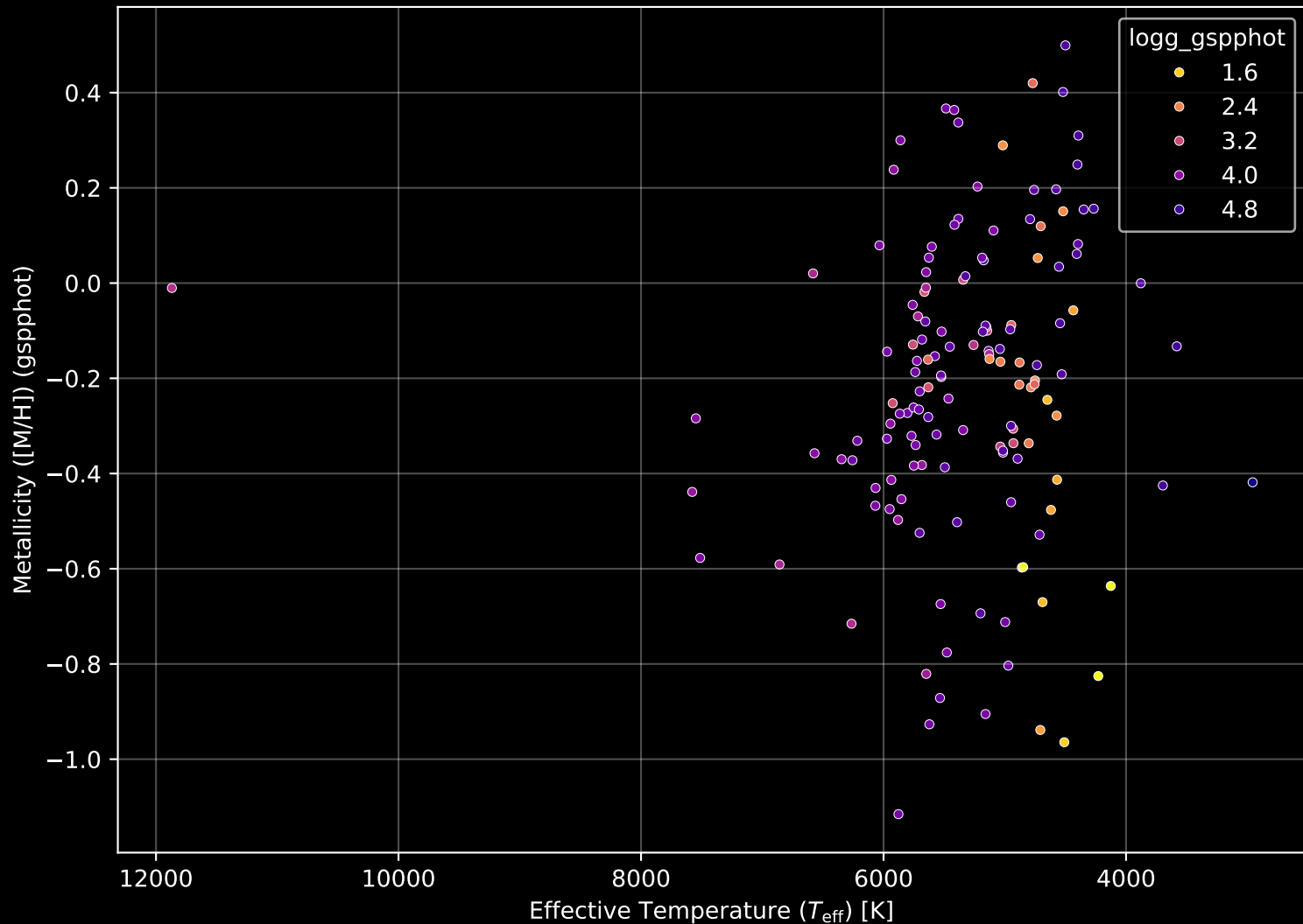
APOGEE DR17 Field: [040+38_MGA] Stellar Population Parameters (n= 143)
